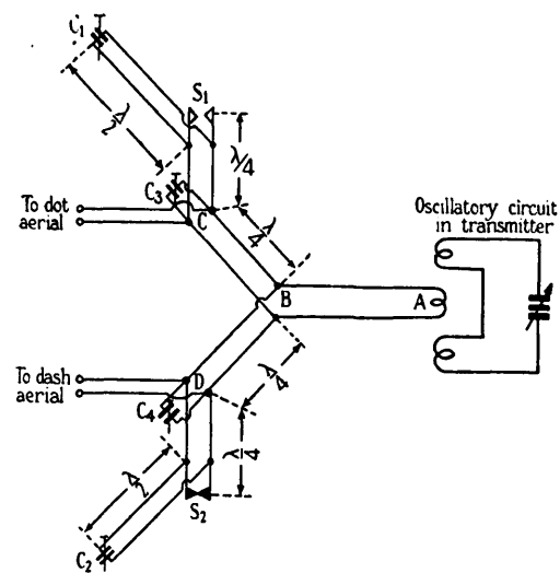
Fig. 4.—Experimental aerial-switching arrangement.
