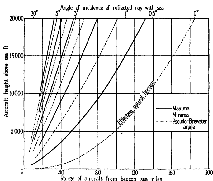
Fig. 3.—Theoretical positions of maxima and minima in the vertical plane for the type-72DP beacon, with aerial height 25λ and vertical polarization.
