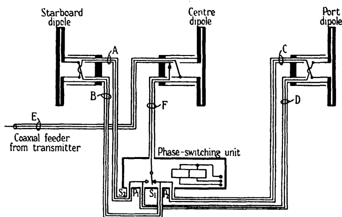
Fig. 6.—Type-93 aerial-feeding arrangements. Cables A, B, C and D are identical in length.
